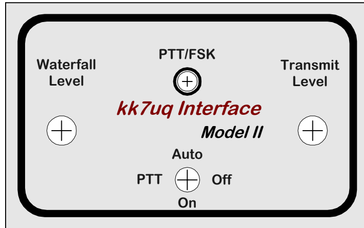
Figure 5.8 Panel Overlay
