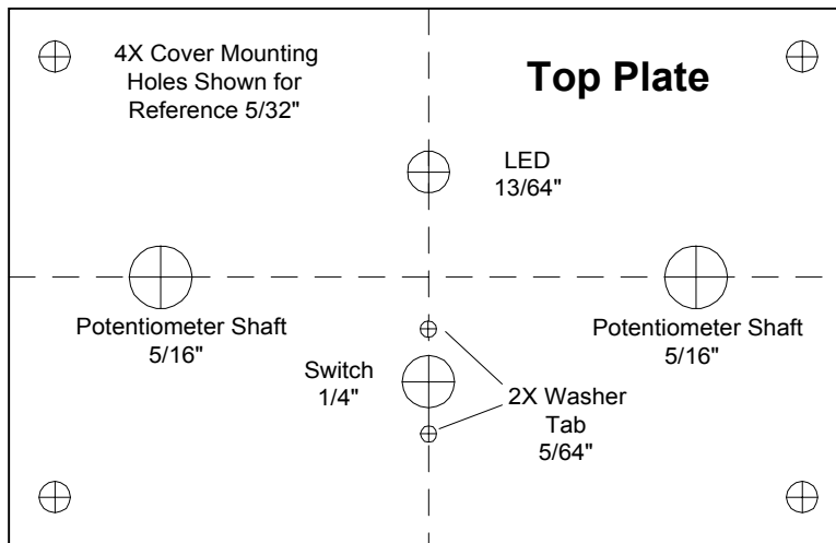
Figure 5.11 Cover Drill Templates
