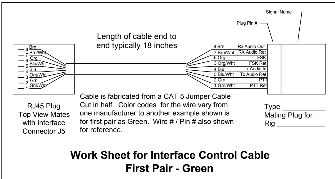
Figure 5.7 Work Sheets for Interface Control Cable
