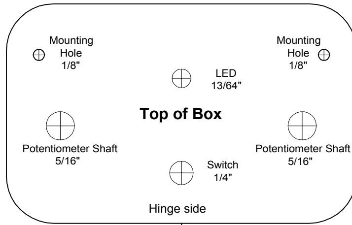
Figure 5.6 Altoids ® Cover Drill Templates
