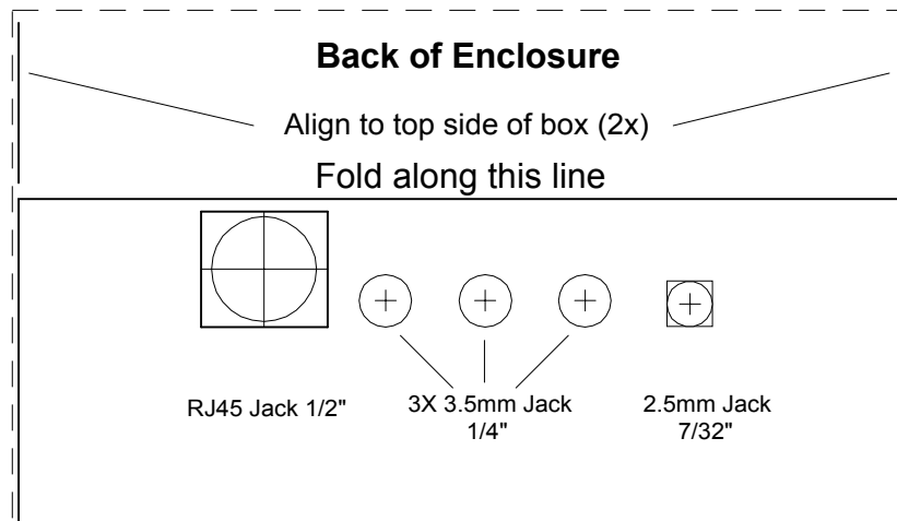
Figure 5.13 Enclosure Template
