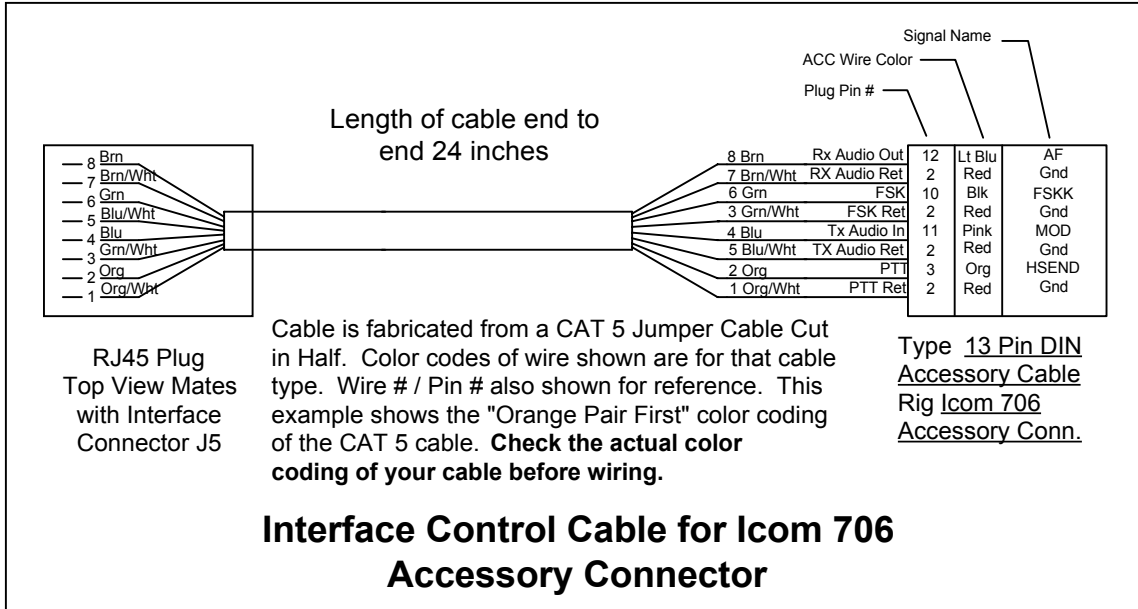
Figure 5.5 SSB Rig Control Cable Connected to the Accessory Port
