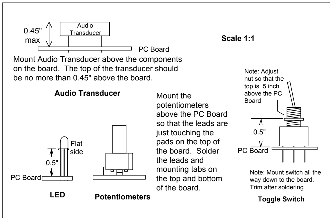
Figure 5.1 Component Mounting
