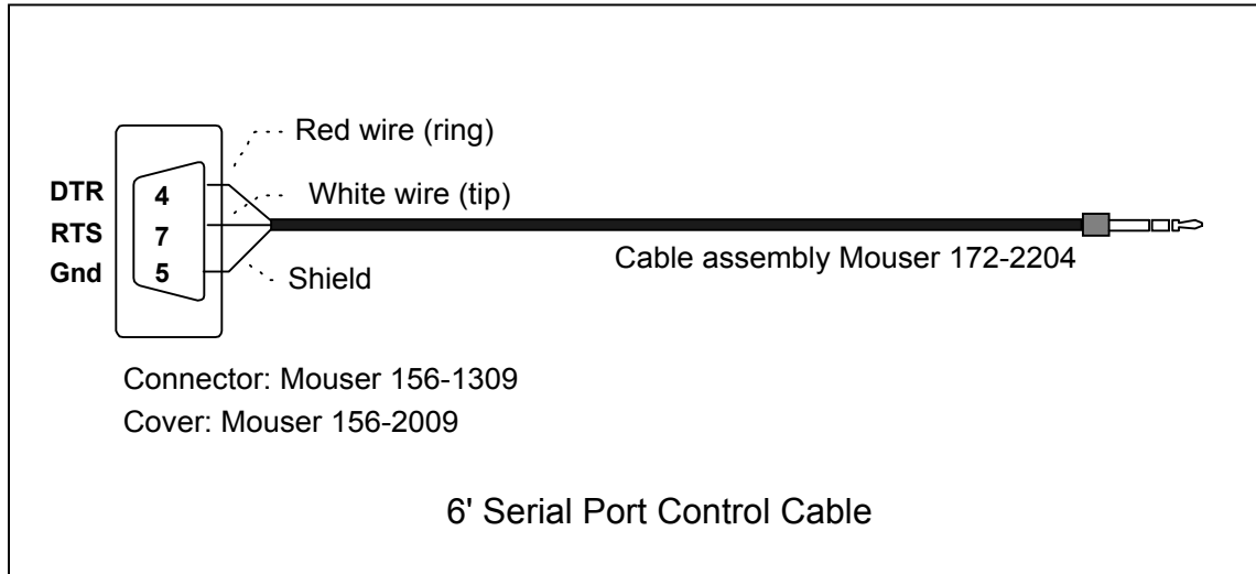
Figure 5.4 Serial Port Control Cable
