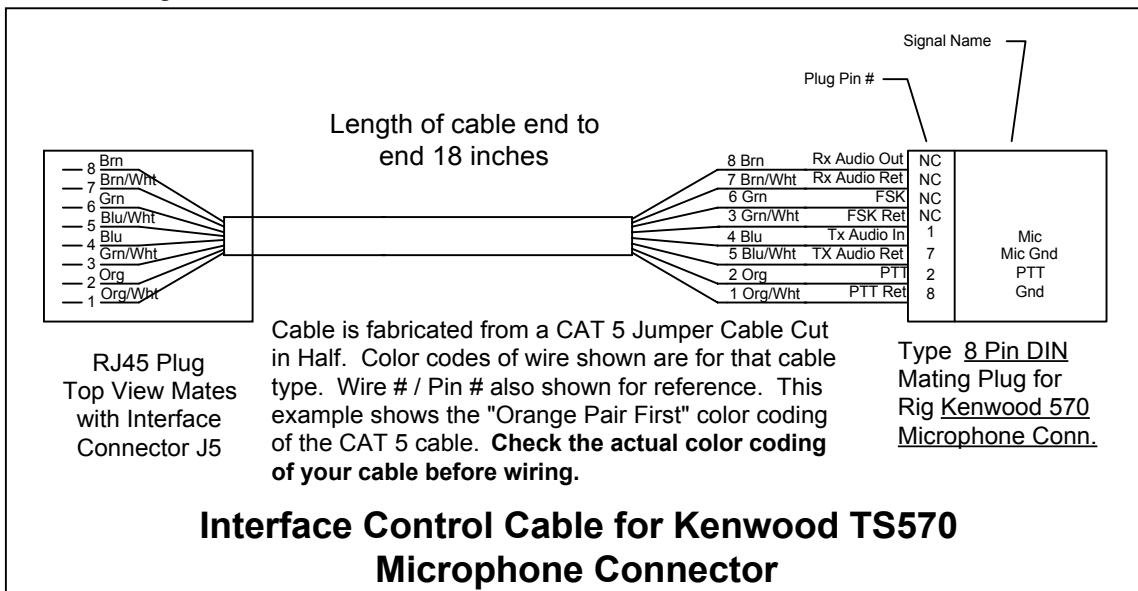
Figure 5.6 SSB Rig Control via the Microphone Connector
